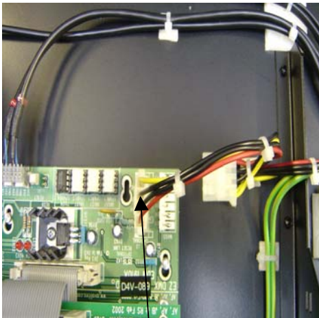
EZ DMX BOARD D/DRIVE CONNECTOR (POWER)
